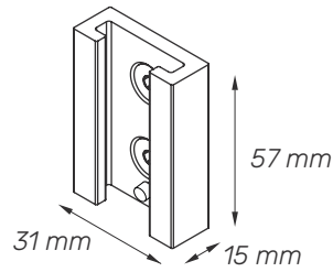
Humidifier mount
